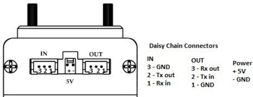
Figure 2.3 (Rear Panel).
