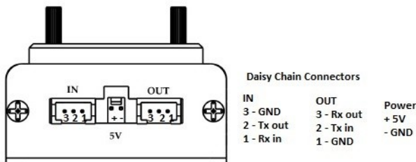
Figure 4.11 (3A-6A & 3RGB-6RGB)
