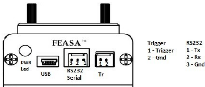
Figure 2.2 (Front Panel).
