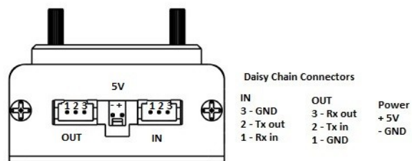
Figure 4.12 (10A & 10RGB).
